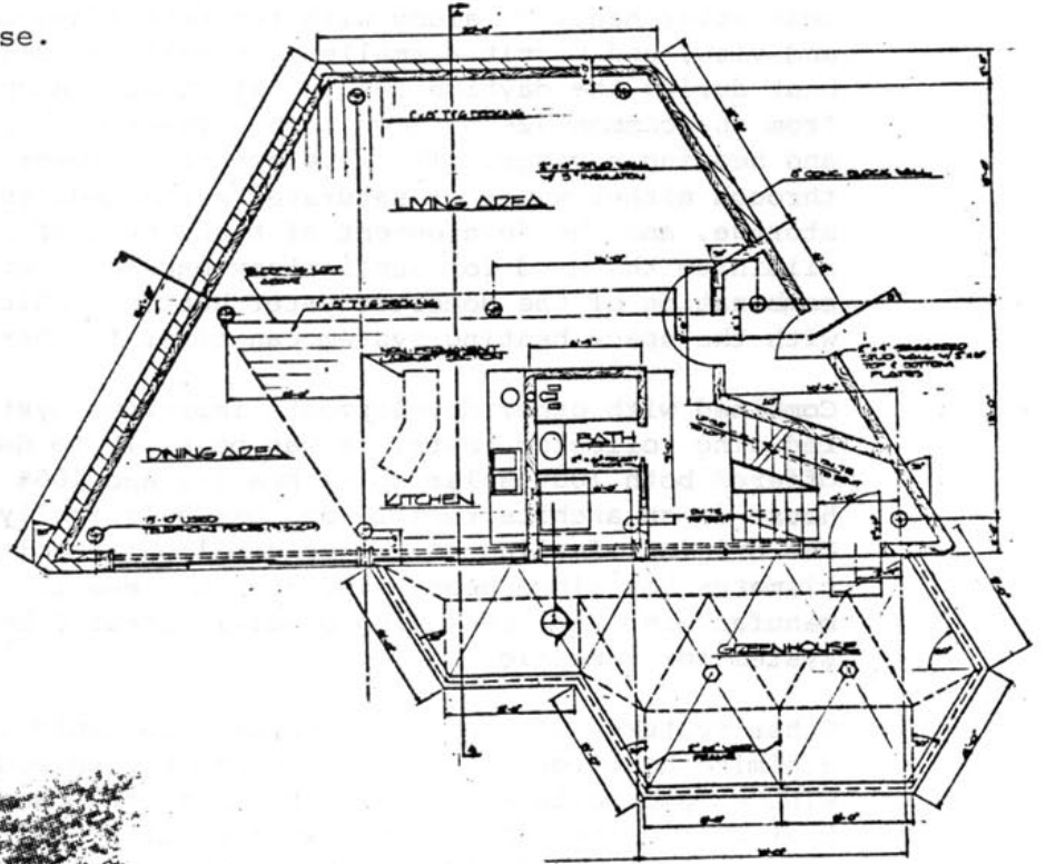
Main floor plan (loft above).
