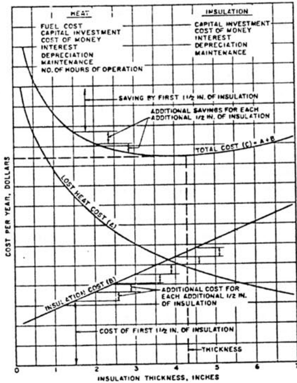
Determination of economic thickness of insulation.
