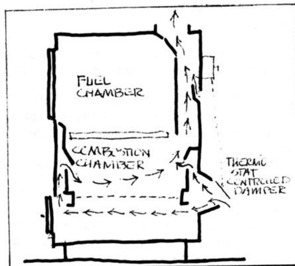
Downdraft wood burner.
